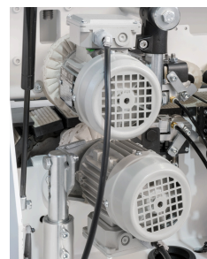
Buffing station
